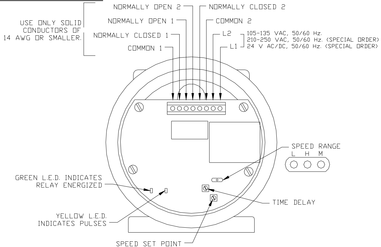
FIGURE 4: Electronics View
